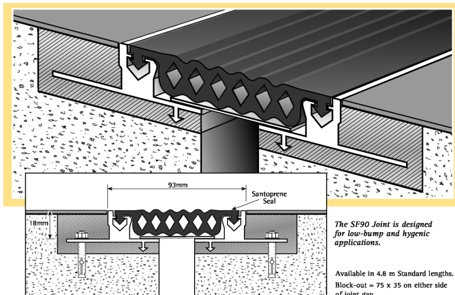
SF90 Fully Sealed and Colour Matched Joint
